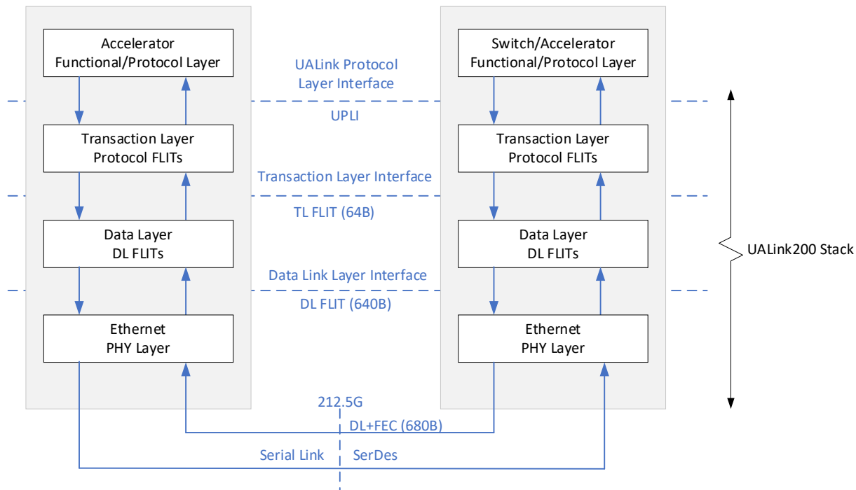
Figure 4: UALink Stack
