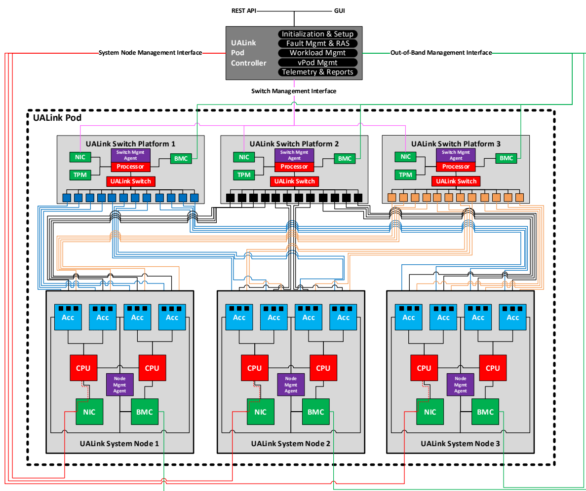
Figure 10: UALink Rack Scale system management interface
